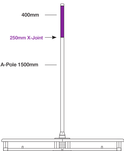
Total height: 1900mm - 74.8" Room Height Needed - 2035mm (80.1")
