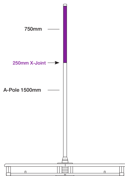
Total height: 2250mm - 88.6" Room Height Needed - 2385mm (93.9")
