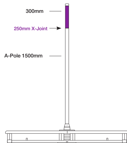
Total height: 1800mm - 70.9" Room Height Needed - 1935mm (76.2")
