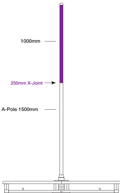
Total height: 2500mm - 98.4" Room Height Needed - 2635mm (103.7")
